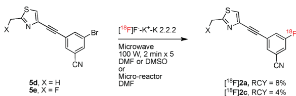
Scheme 2 Syntheses of [ ^{18}F ] 2a and [ ^{18}F ] 2c via nucleophilic substitution in bromo precursors 5d and 5e , respectively.
