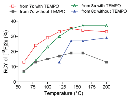
Fig. 1 Effects of aryl partner and TEMPO on RCY of [ ^{18}F ] 2c in the microfluidic apparatus from precursors 7c (aryl partner: Ph) and 8c (aryl partner: 4-MeOC 6 H 4 ).
