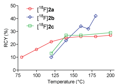
Fig. 2 Temperature dependence of RCYs of [ 18 F]2a–c from 8a–c , respectively, in the microfluidic apparatus. Residence times were 251 (○), 188 (◇) and 251 s (□).
