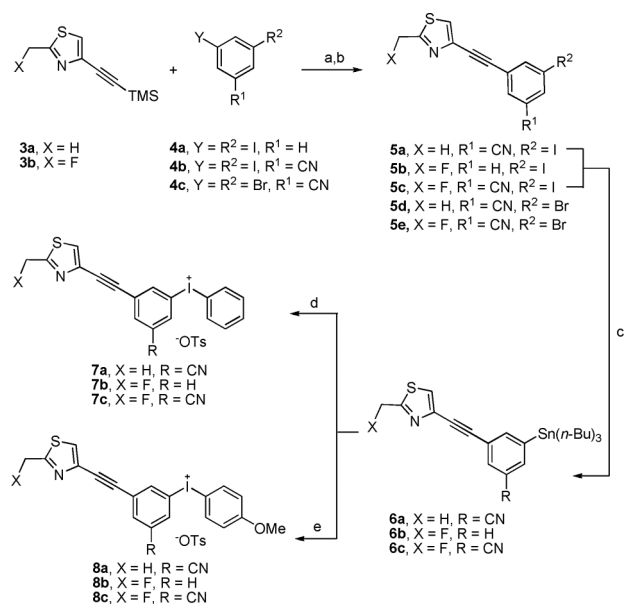
Scheme 1 Syntheses of bromo-precursors 5d and 5e , and the diaryliodonium tosylates 7a–c and 8a–c . Reagents and conditions: (a) Pd(PPh 3 ) 4 or Pd(PPh 3 ) 2 Cl 2 , CuI, Et 3 N, DME; (b) 1 M ( n -Bu) 3 NF in THF, 80 °C; (c) Sn 2 ( n -Bu) 6 , Pd(PPh 3 ) 4 , toluene, 115 °C, 16–24 h; (d) Koser's reagent, CH 2 Cl 2 , r.t., 24–48 h; (e) 1-(diacetoxyiodo)-4-methoxybenzene, p -TsOH·H 2 O, MeCN, CH 2 Cl 2 , r.t., 24 h.
