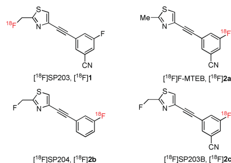
Chart 1 Structures of [ ^{18}\text{F} ]SP203 and target radioligands.
