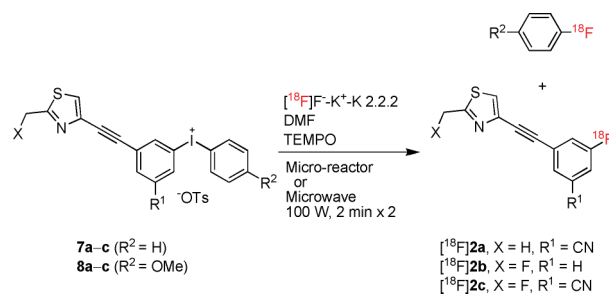
Scheme 3 Radiosyntheses of target radioligands [ ^{18}F ] 2a–c from diaryliodonium tosylates.
